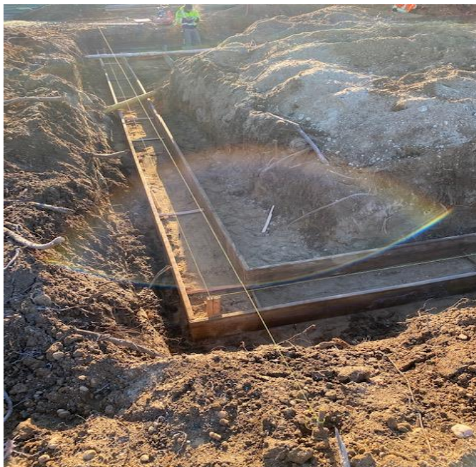
Excavation for the Fieldhouse addition commenced at High School East. Footings are formed and awaiting concrete pour.
